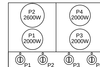
COMMUTATOR POSITIONS
