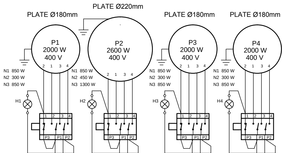
COMMUTATOR POSITIONS
