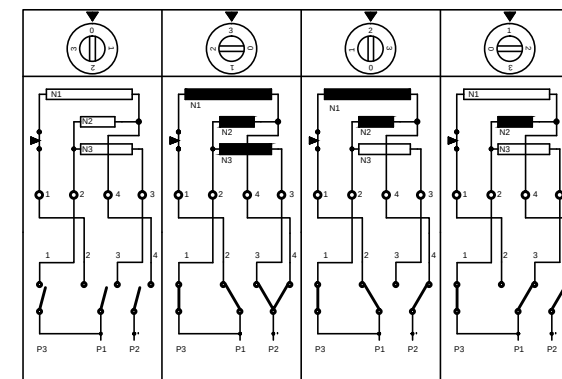
STEATITE COMMUTATOR POSITIONS
